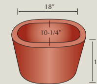
10 x 17 Oval Flue Liner
